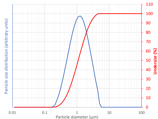
Typical particle size distribution. (Laser diffraction method.)
